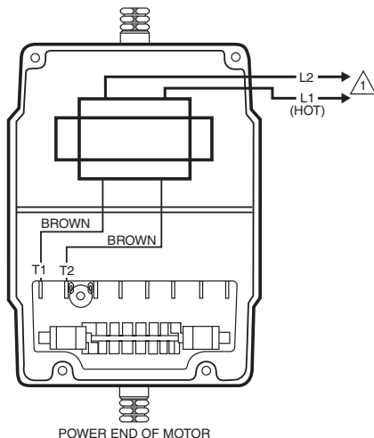
Fig. 1. Mounting 50017460 transformer in Modutrol IV Series 2 Motor.
